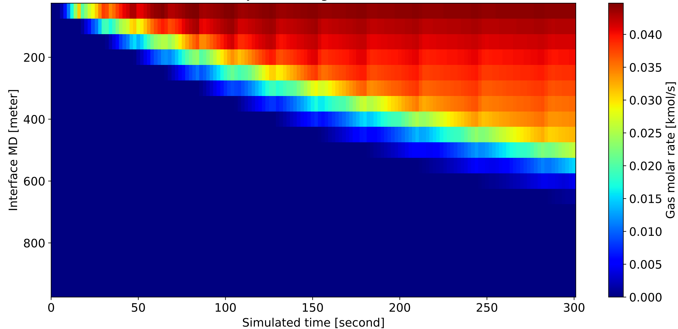
Gas molar rate profile along the wellbore over time
